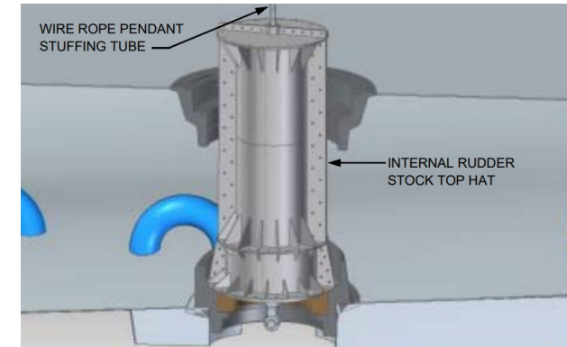
Internal cofferdam assembly
