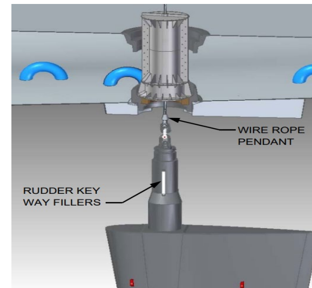
Rudder/stock rigged/raised under hull
